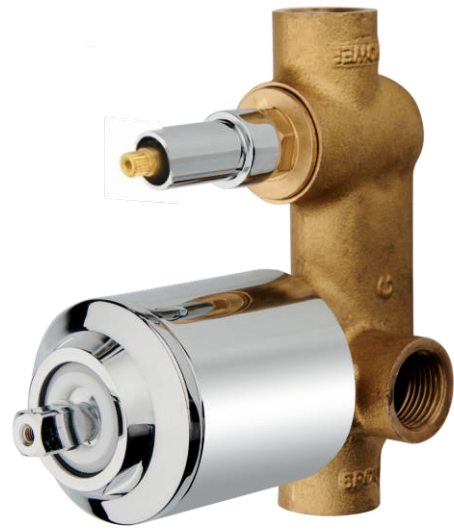
DIV-562 4 WAY DIVERTER BODY HIGH FLOW 45mm
